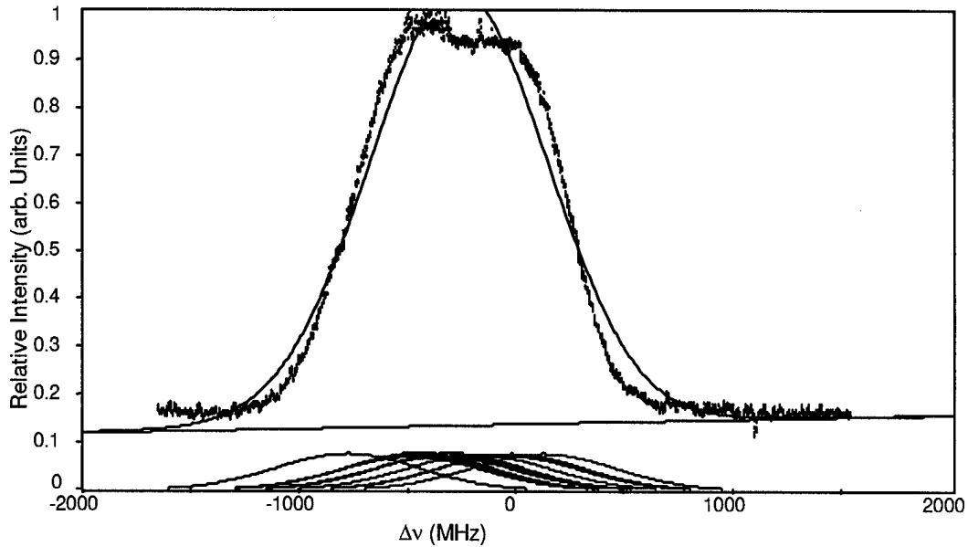
Figure C-4. P(70) 17-1 Doppler-broadened transition at the 4 " position of the Phase II cell, measured using Doppler-limited saturation spectroscopy. SNR=143.8, mean baseline=0.0169 +/- 0.00696, R^2=0.978 , FWHM = 774.3 MHz, Extracted Temperature=1099 K
