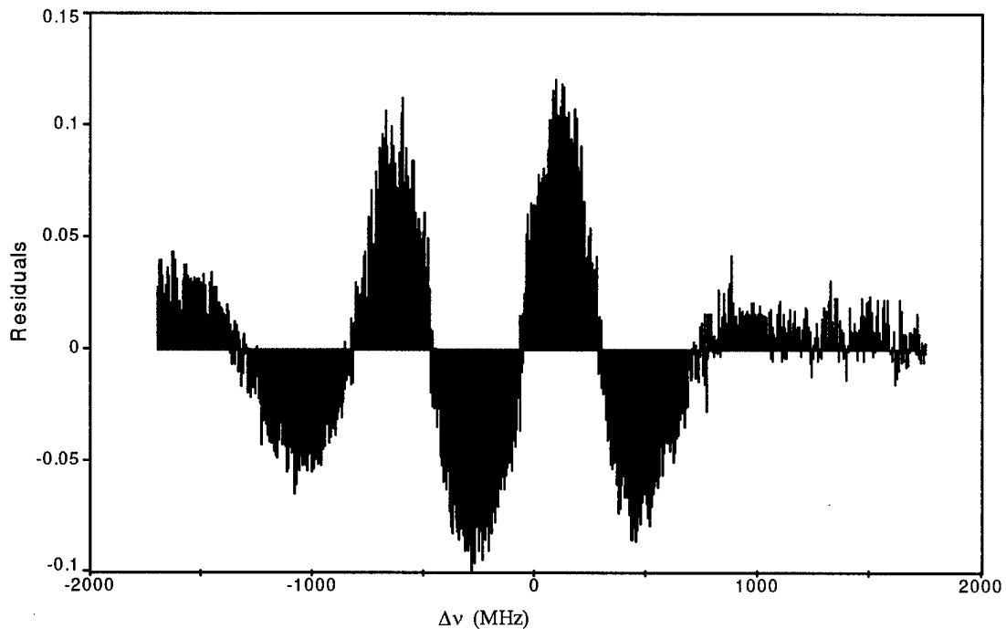
Figure C-7. P(70) 17-1 residual trend for the 3 " Doppler-limited fit.
