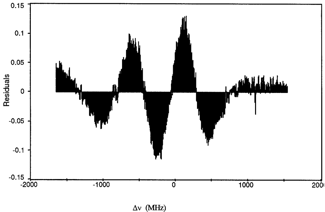
Figure C-5. P(70) 17-1 residual trend for the 4 " Doppler-limited fit.
