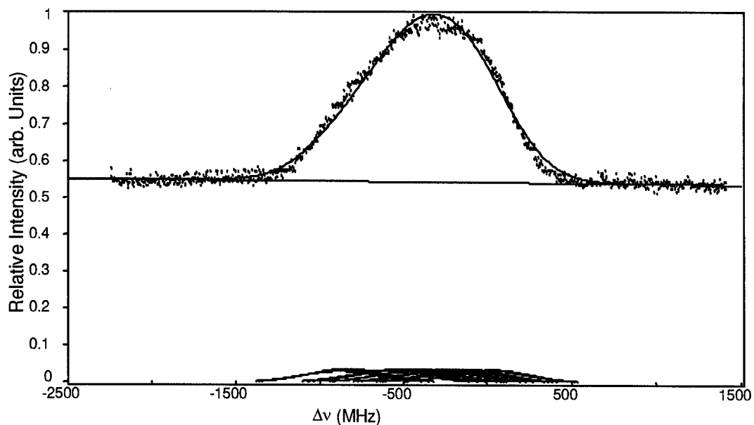
Figure C-12. P(53) 19-2 Doppler-broadened transition at the 4 " position of the Phase II cell, measured using Doppler-limited saturation spectroscopy. SNR=99.2, mean baseline=0.567 +/- 0.101, R^2=0.99 , FWHM = 555.8 MHz, Extracted Temperature=566 K
