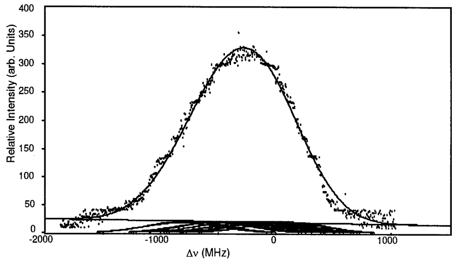
Figure C-3. P(53) 19-2 Doppler-broadened transition at the cot end of the Phase I cell, measured using Doppler-limited saturation spectroscopy. SNR=34.0, mean baseline=14.4 +/- 9.7, R^2=0.989 , FWHM =775 MHz, Extracted Temperature=1102 K
