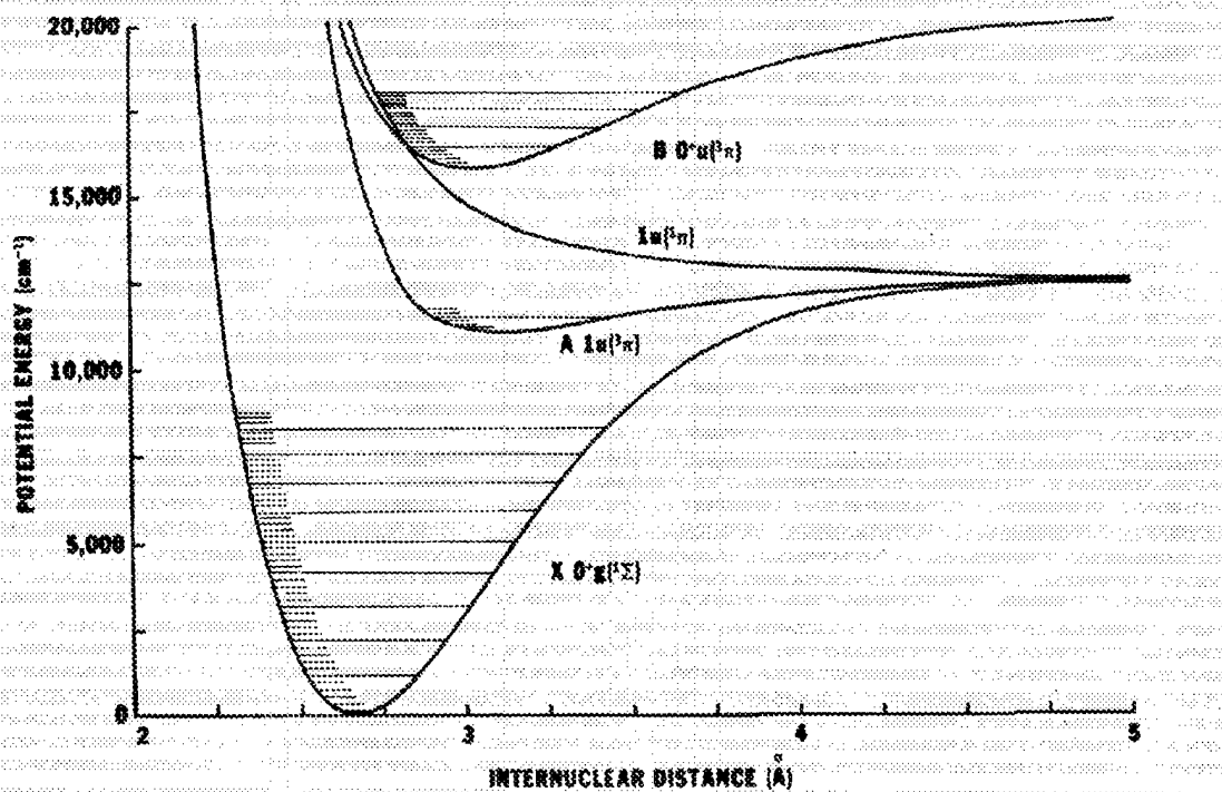
Figure 7. Energy level structure for the first few electronic levels in I_2 . Note that the B state has significant predissociation caused by the crossing of a repulsive potential level. 16
