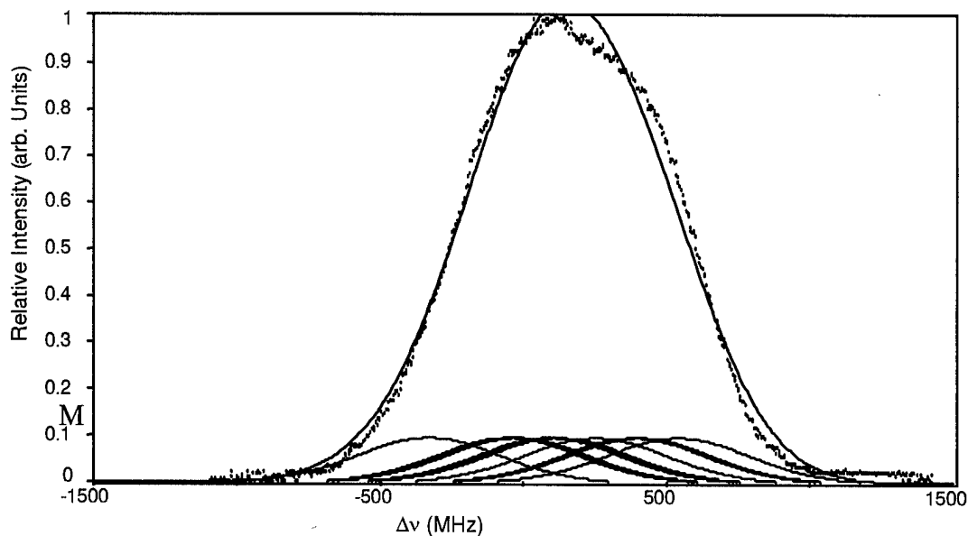
Figure 36. P(70) 17-1 Doppler-broadened transition at the cold end of the Phase I cell, measured by Doppler-limited saturation spectroscopy. SNR=122.5, mean baseline=18.5 +/- 13.6, R^2=0.993 , FWHM=581 MHz, Extracted Temperature=615 K
