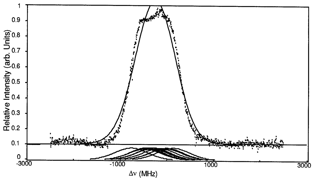
Figure C-10. P(70) 17-1 Doppler-broadened transition at the 1 " position of the Phase II cell, measured using Doppler-limited saturation spectroscopy. SNR=64.4, mean baseline=0.114 +/- 0.0155, R^2=0.98 , FWHM = 827.2 MHz, Extracted Temperature=1254 K
