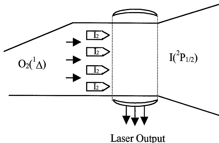
Figure 2. COIL nozzles and optical cavity. The I_2 is injected through the supersonic nozzles and dissociates, allowing for the resonant energy transfer from the excited oxygen to the atomic iodine. The lasing transition occurs aft of the nozzles in the resonant laser cavity. 3
