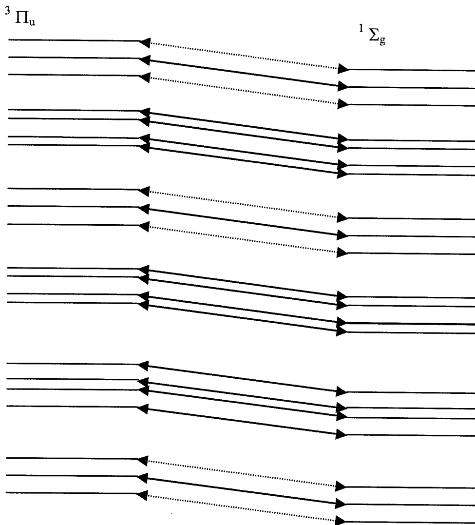
Figure 8. Hyperfine transitions in I_2 . In each electronic state the individual splittings are due to the possible quantized F-values. The dotted lines designate transitions that do not occur for even J'' interactions, such that there are 21 odd J'' hyperfine transitions and 15 even J'' hyperfine transitions. 19
